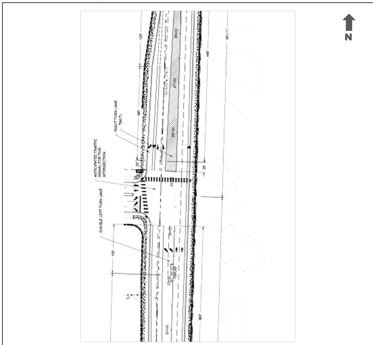
Figure 1. Proposed Configuration of 228 th Avenue SE / Site Access Driveway Intersection
